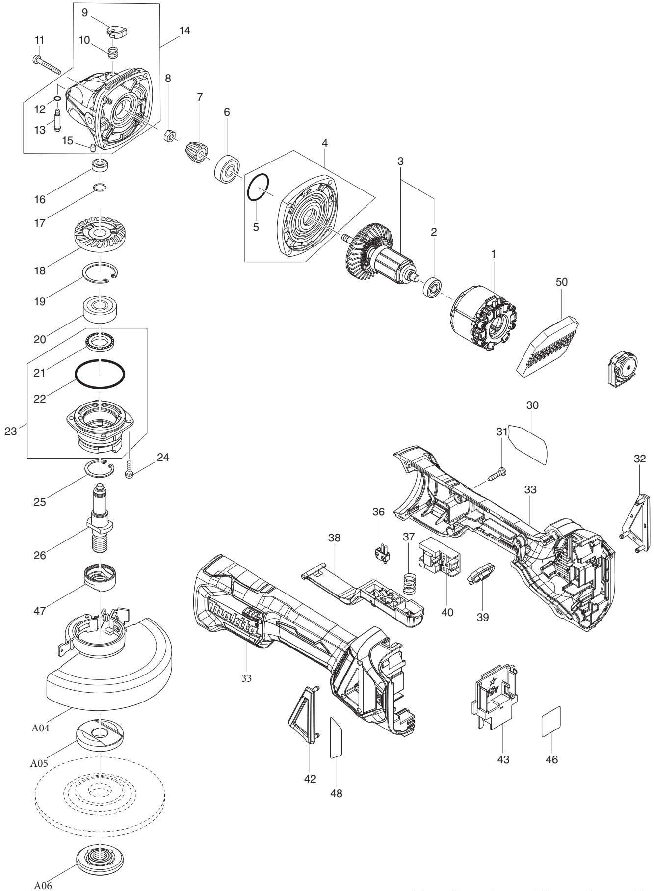
DGA517 - 18V LXT Brushless 5" Grinder, Paddle Switch, Variable speed
