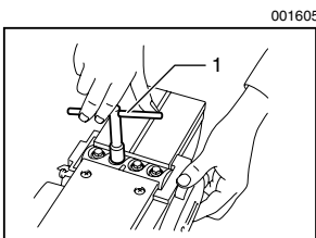
1. Socket wrench
